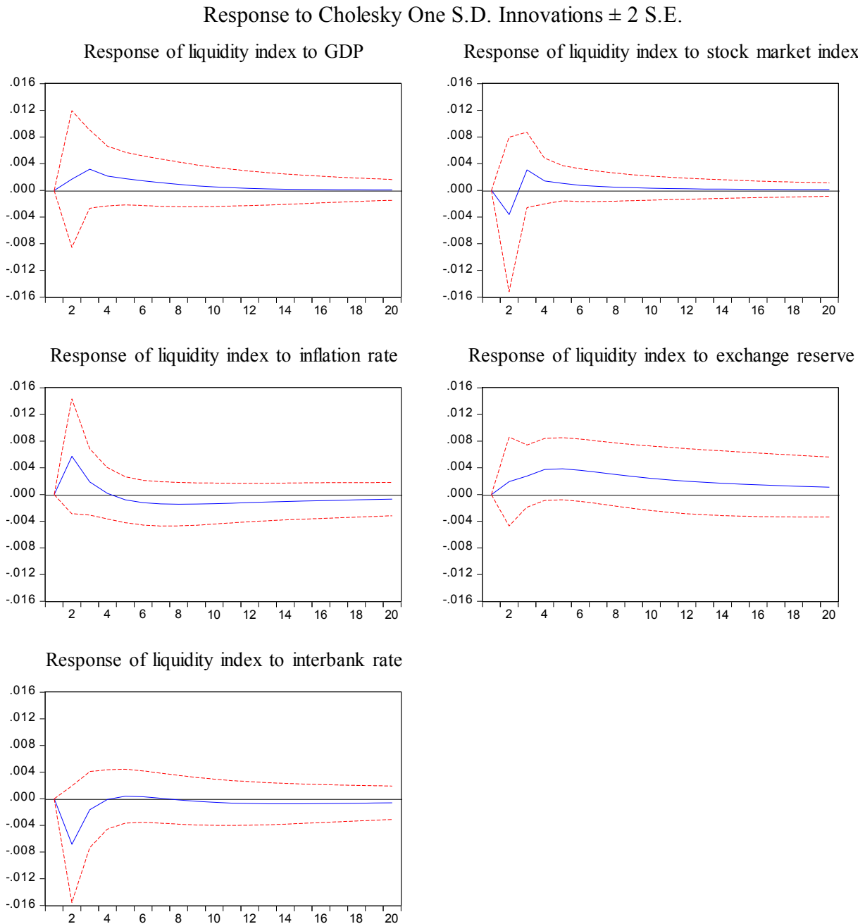
Figure 7: impulsion responses (VAR model)
